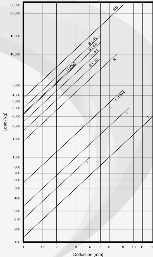
LOAD DEFLECTION CURVES HIGH LOAD MOUNTS
