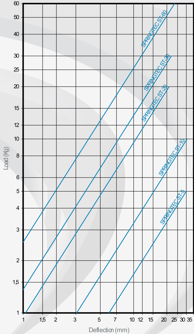
LOAD DEFLECTION GRAPH AMC MECANOCAUCHO SPRINGTEC
